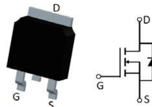
TO-252
